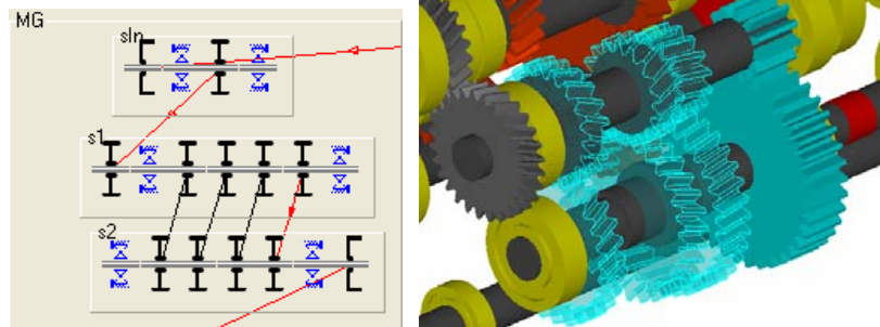
Figure 4.5-1 Gear selections for main gears
