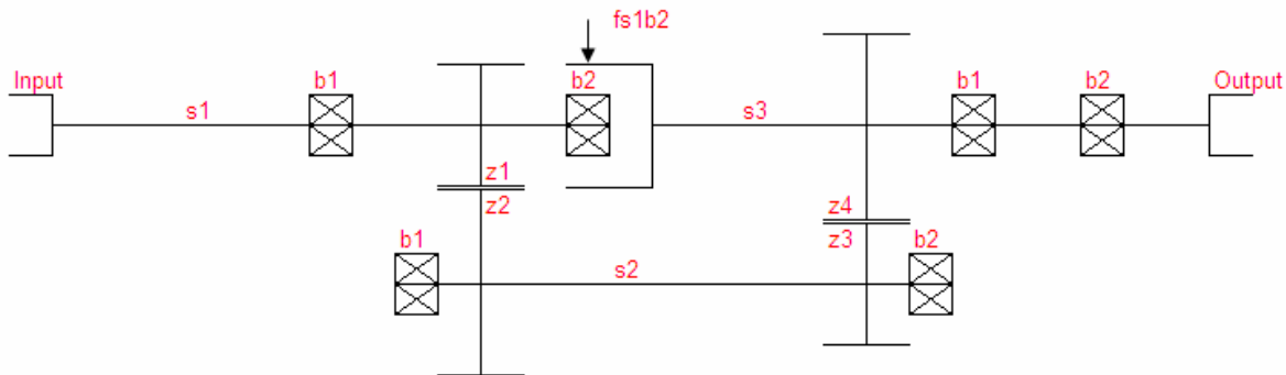
Figure 4.6-3 Schematic of a pilot bearing model in KISSsys.
